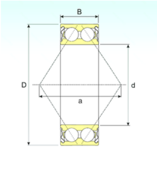
5310ZZ Bearing 2D drawings and 3D CAD models
