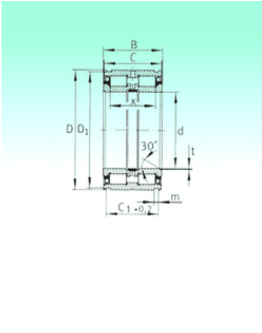
SL04130-PP Bearing 2D drawings and 3D CAD models
