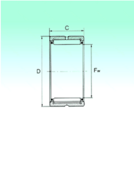
NKS 60 Bearing 2D drawings and 3D CAD models
